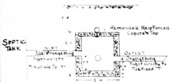
SECTION
